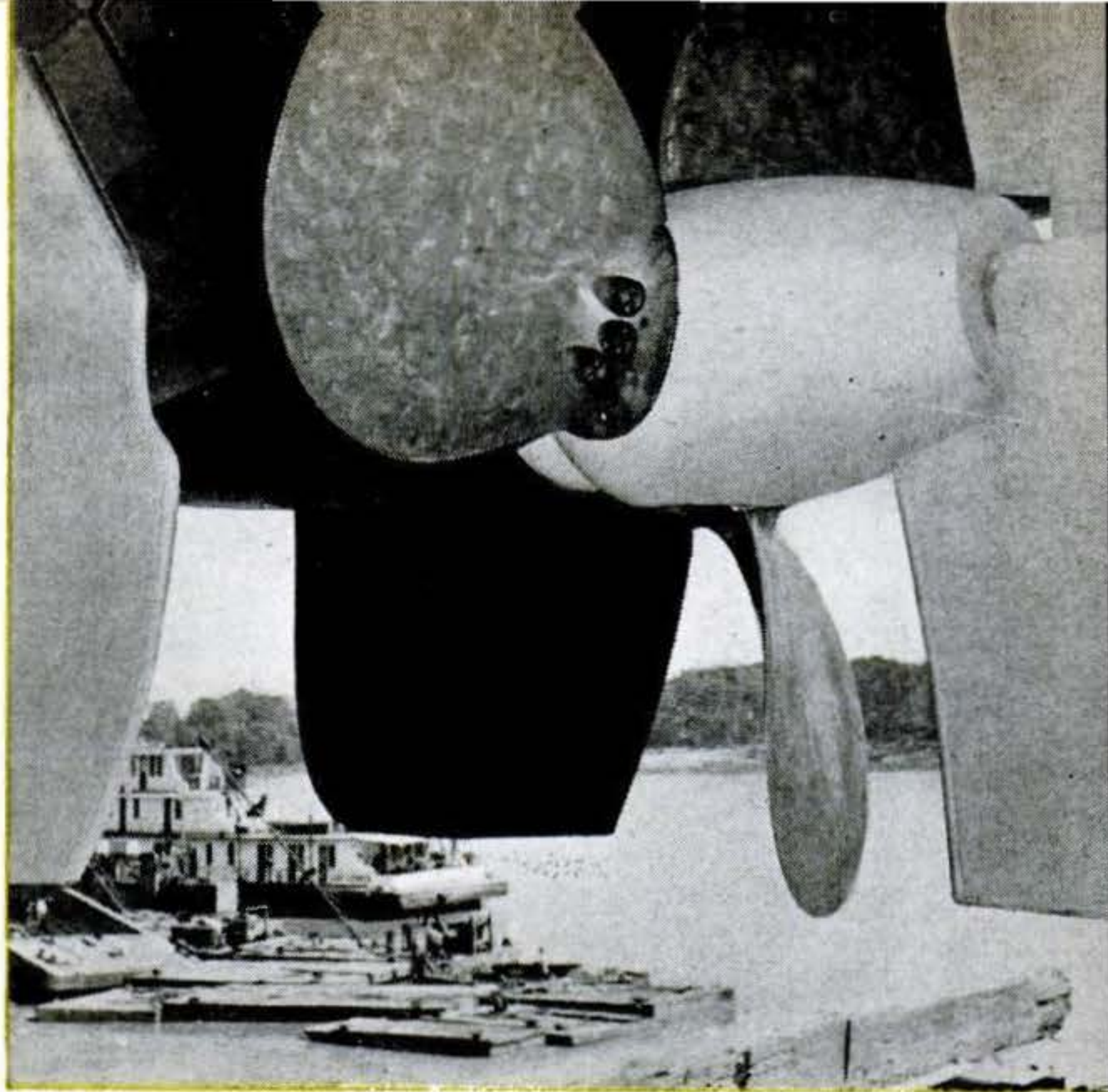
PRELAUNCHING VIEW shows one of nine-foot-diameter, stainless-steel twin screws, believed largest of variable pitch in U. S., that propel 3,200-hp. Diesel towboat Delta Cities .
